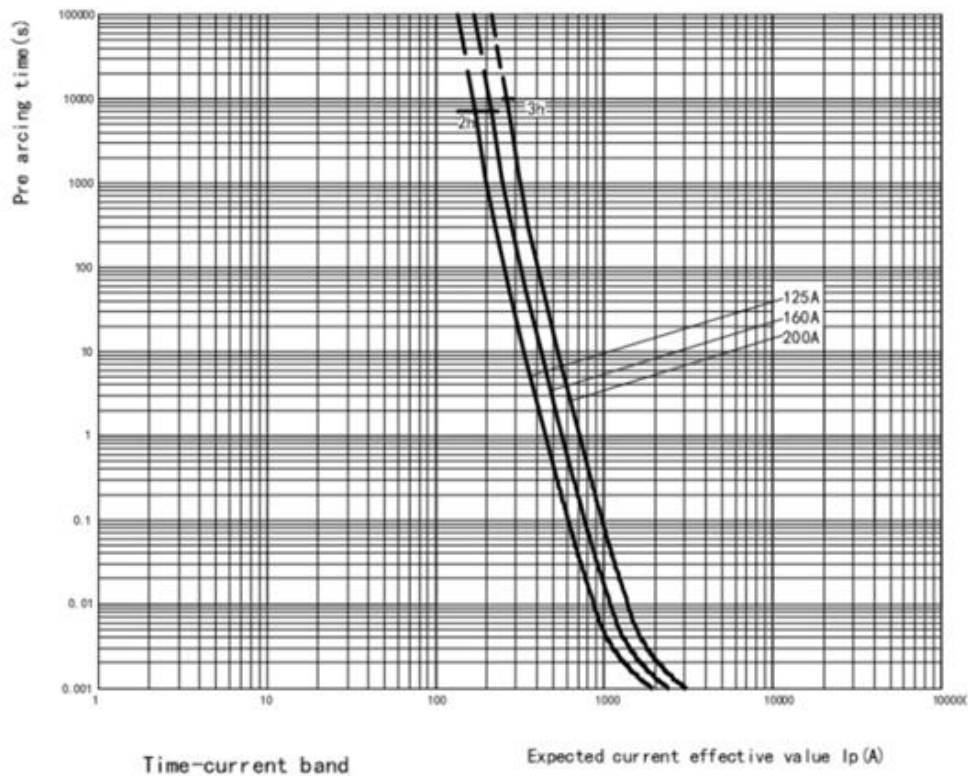
FIG. 1、 Forearc time - expected current curve
