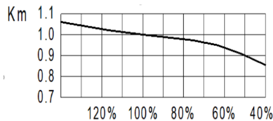
Connection wire cross section/Standard cross section
