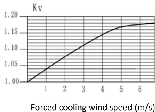
FIG. 4、 correction coefficient of wind speed and rated current – K_v
